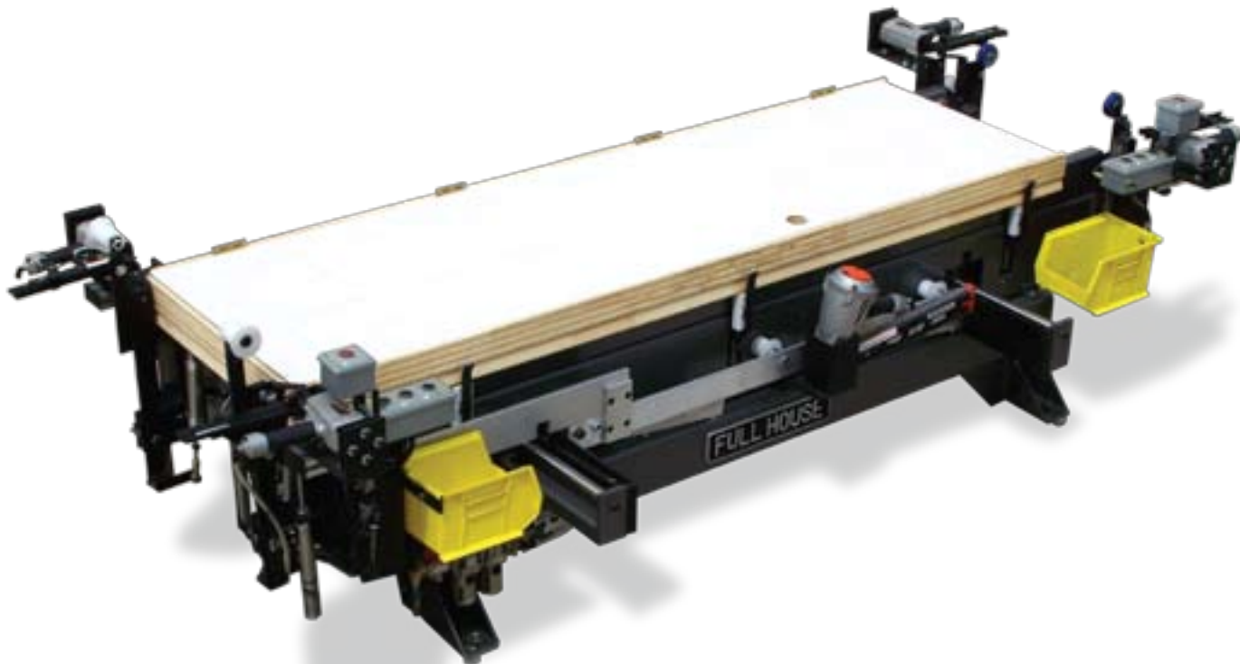
Jambs are securely clamped during stapling.
